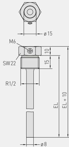
Dimensional drawing TH08- ms /xx
