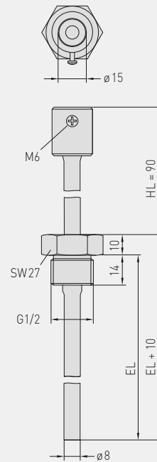
Dimensional drawing TH08- VA /xx/90
